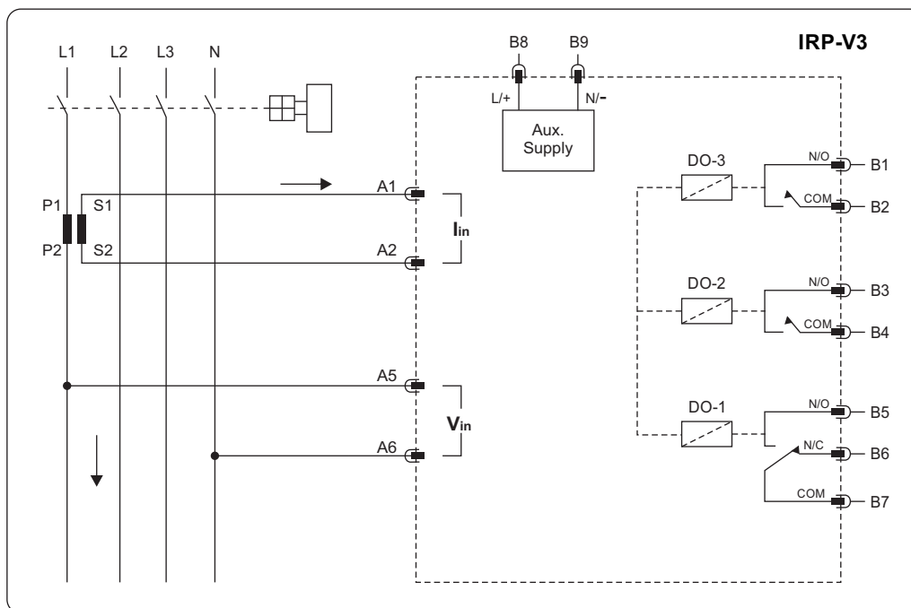
Connection Line to Neutral Voltage in 3 Phase, 4 Wire System (Default Connection)
