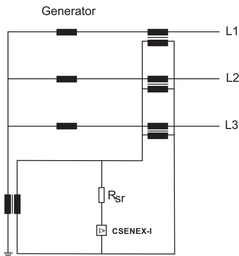
Zero current differential protection of the star point winding (restricted earth fault 64REF) of a generator
