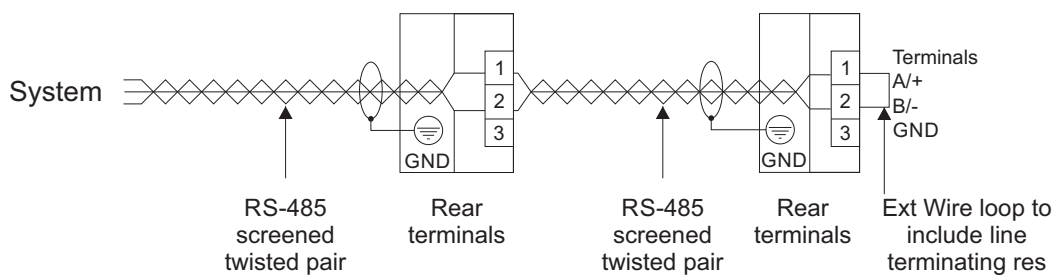
Communication to multiple devices from control system using RS-485
