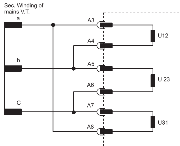
Fig. 4.1: Input v.t.s in delta connection ( \Delta )
