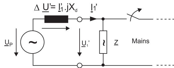
Fig. 4.6: Equivalent circuit at mains failure
