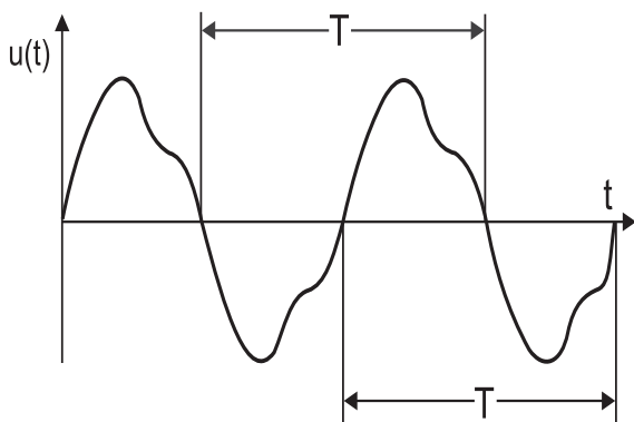
Fig. 4.3: Determination of cycle duration by means of zero passages.
