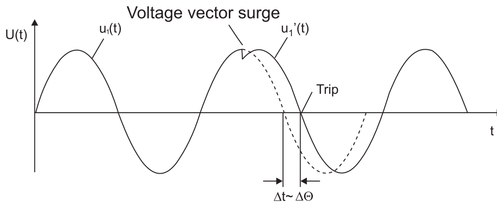
Fig. 4.8: Voltage vector surge
