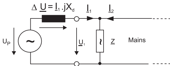
Fig. 4.4: Equivalent circuit at synchronous generator in parallel with the mains
