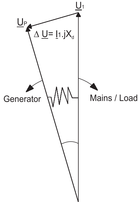
Fig. 4.5: Voltage vectors at mains parallel operation
