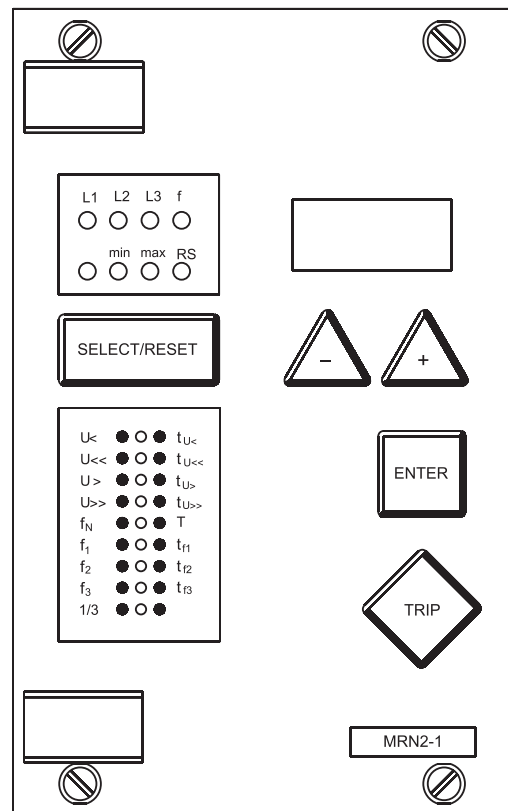
Fig. 3.2: Front plate MRN2-1
