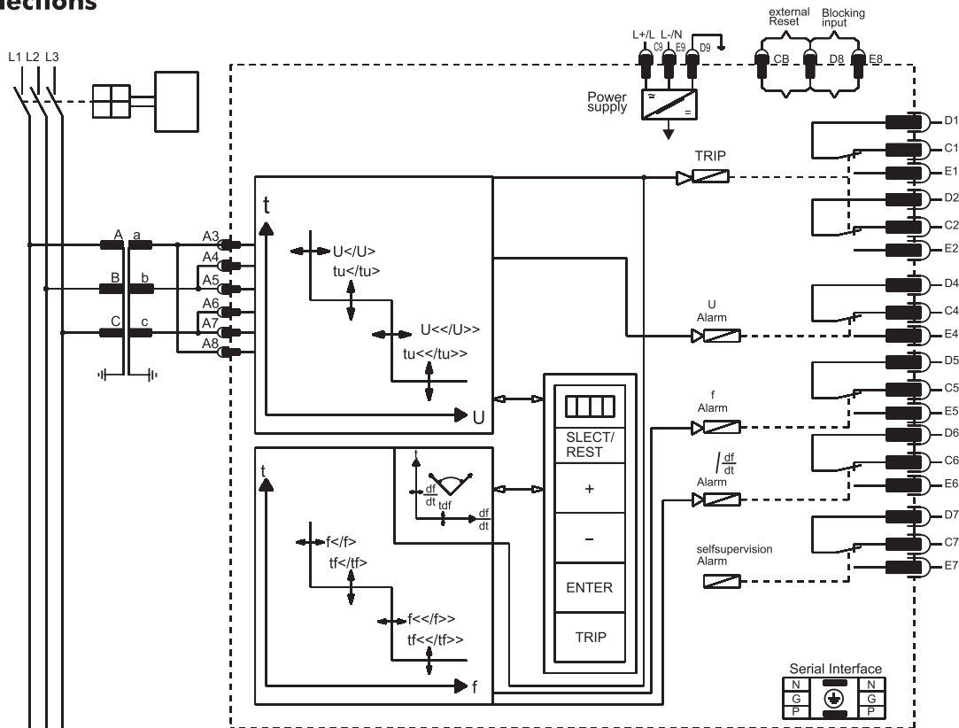
Fig. 3.1 : Connection diagram MRN2-1 and MRN2-2
