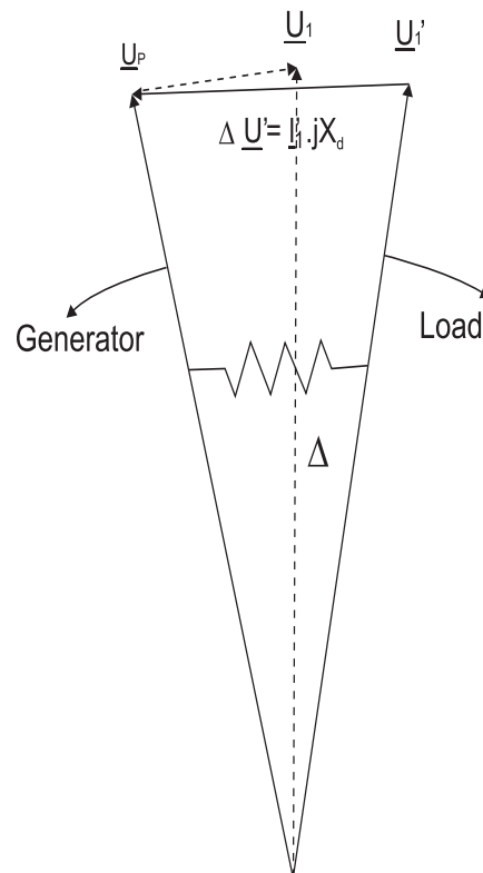
Fig. 4.7: Voltage vectors at mains failure
