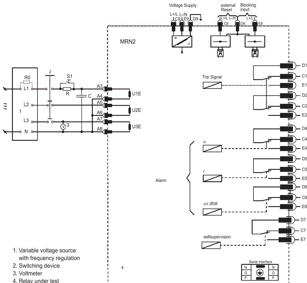
Fig. 6.2: Test circuit for the vector surge function
