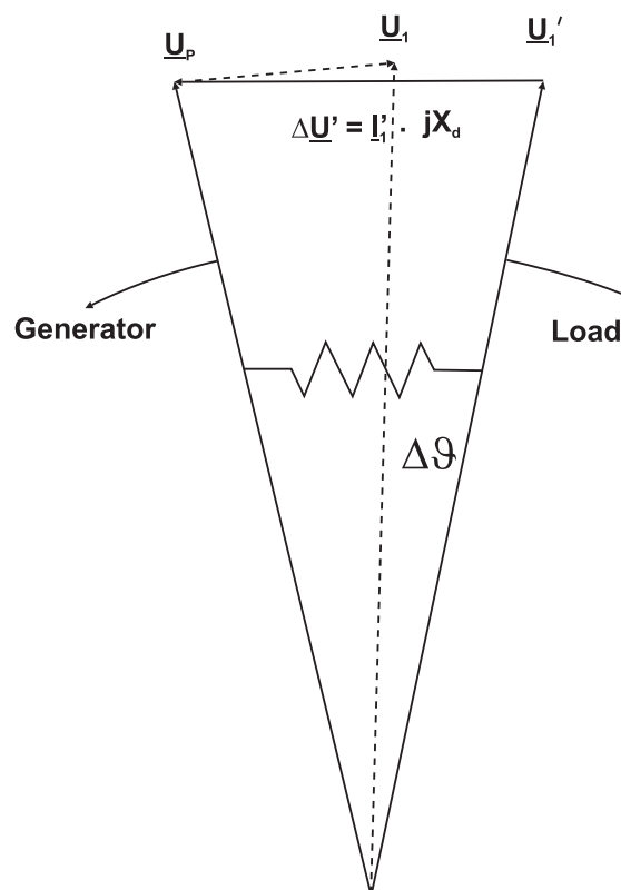
Fig. 4.4: Voltage vectors at mains failure
