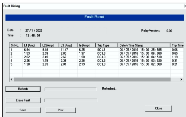
(Fault Data Recording on PC Software)
