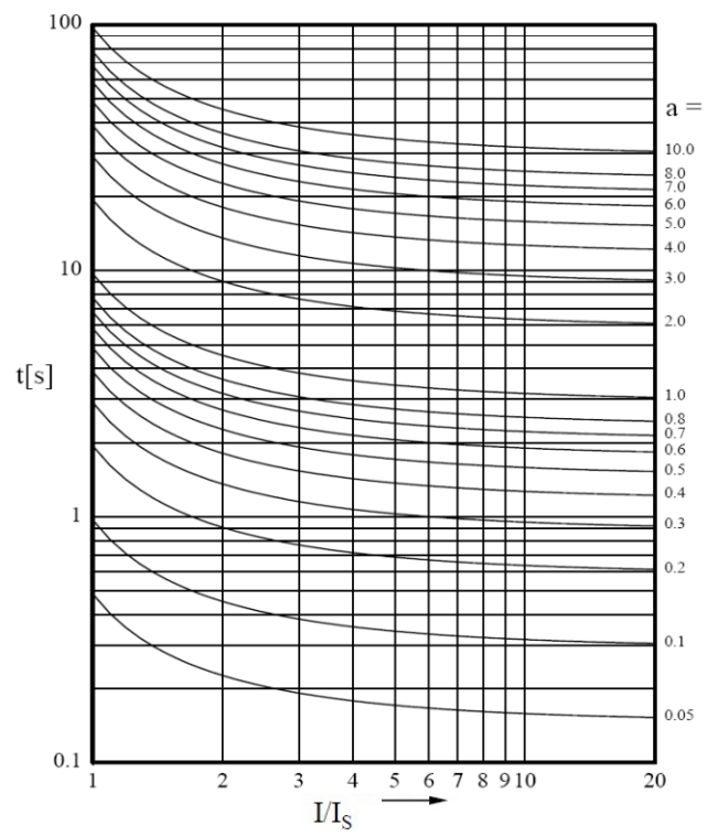
RI-Inverse
