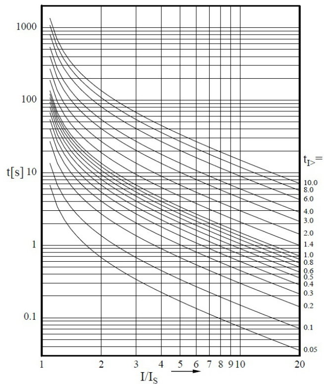
Very Inverse
