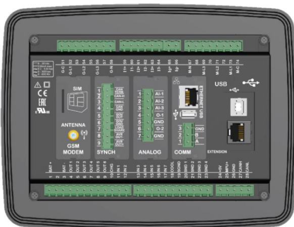
Backpanel view
