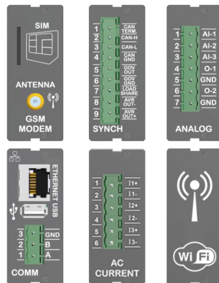
Plug-in modules
