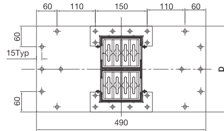
Section X-X'
